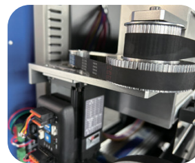
High-Stability Tensioning Pulley System
