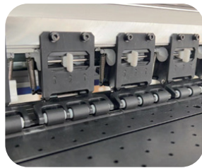
Multi Stage Pinch Roller Structure
